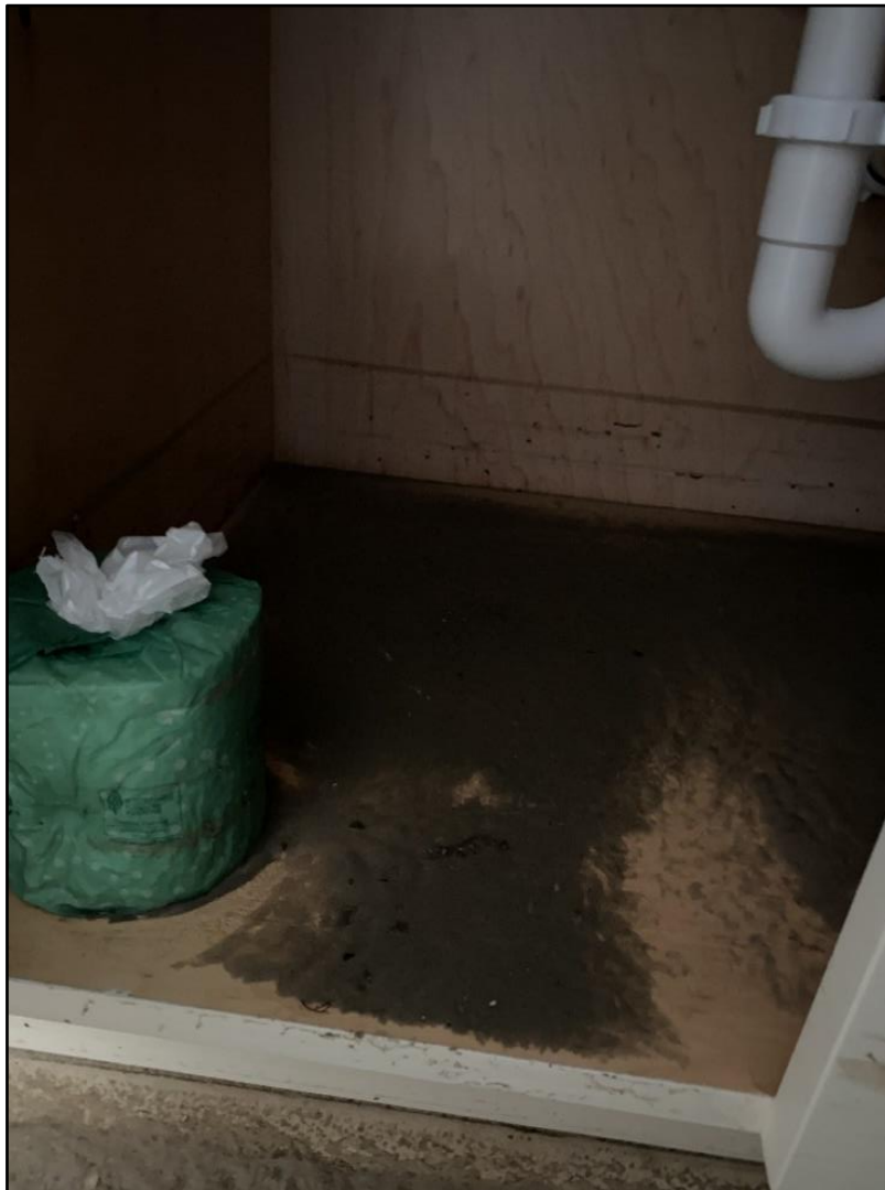
Figure 12. (a) Storm surge high water mark in bathroom cabinet on the second-story of a beachfront structure in Fort Myers Beach. (b) NWS survey team extrapolating the high water mark to the outside of the home to survey its elevation of approximately 12 ft above the brick foundation and 15 ft above MHHW. Images courtesy of the NWS.
